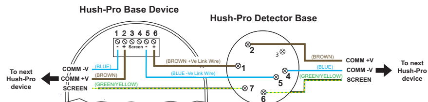
Figure 2 - Connection to Hush-Pro Detector Base (Typical)
