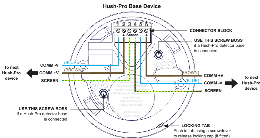
Figure 1 - Connections (Typical)
